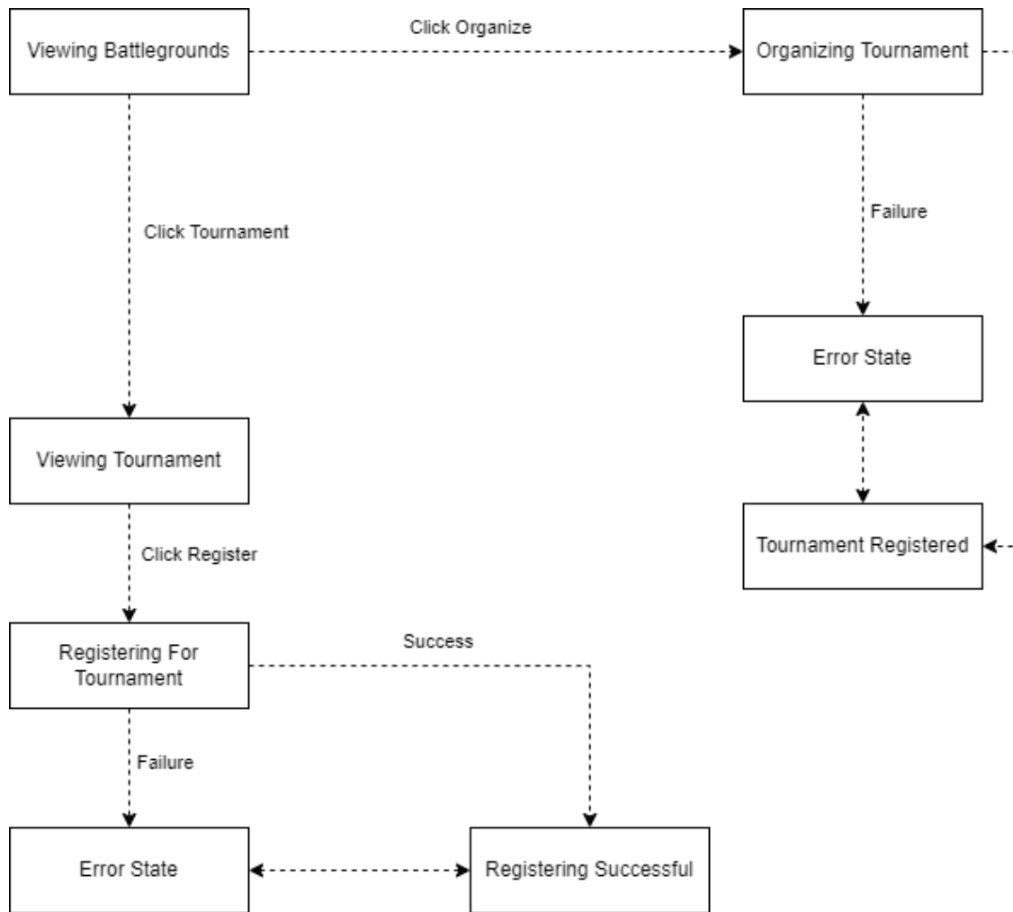
Figure 3.31: Battlegrounds State Transition Diagram
