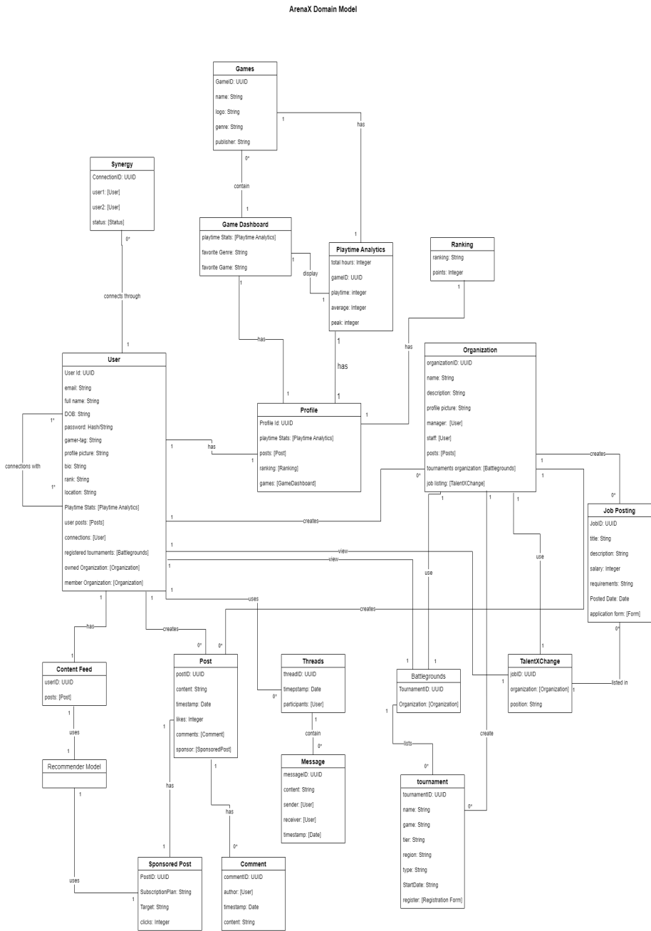
Figure 2.2: ArenaX Domain Model
