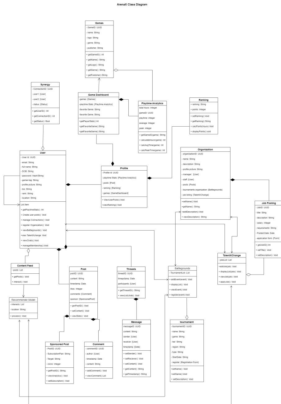
Figure 3.15: ArenaX Class Diagram
