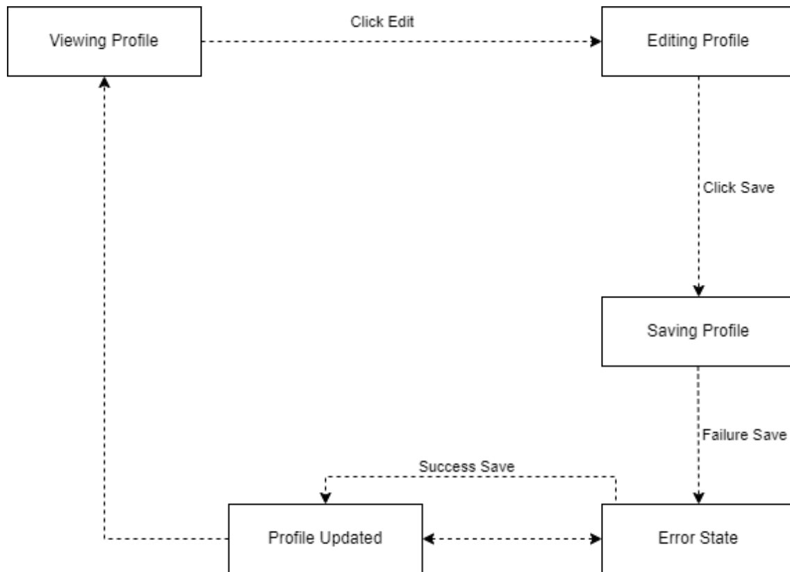
Figure 3.28: User Profile State Transition Diagram
