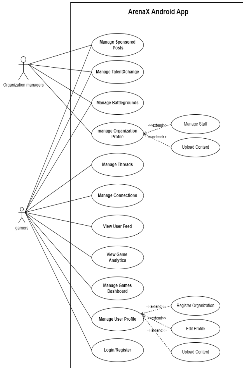
Figure 2.1: ArenaX Use case Diagram
