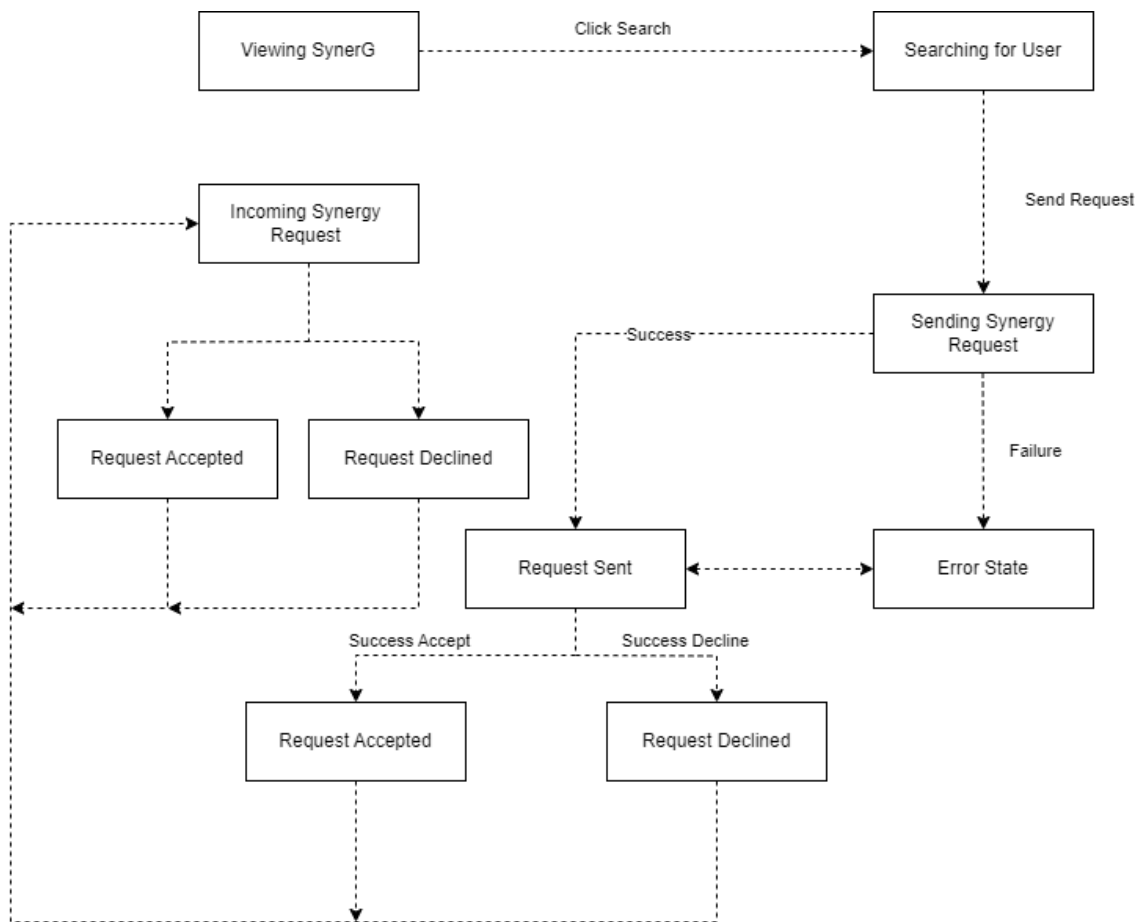
Figure 3.30: Synergy State Transition Diagram
